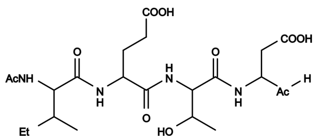
Figure 1. Chemical structure for Ac-IETD-CHO *CAS 191338-86-0*
